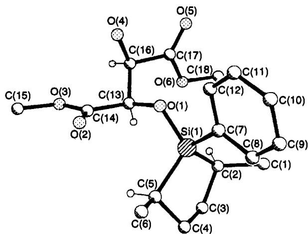
Fig. 1 Molecular structure of the r -1, t -2, t -5-silyl ether 11 derived from L-DMT (only selected hydrogen atoms are shown). Selected bond lengths (Å) and bond or torsion angles (°) are as follows: Si(1)–O(1) 1.653(2), Si(1)–C(2) 1.883(4), Si(1)–C(5) 1.882(3), Si(1)–C(7) 1.863(3), Si(1)–O(1)–C(13) 128.2(2), C(2)–Si(1)–C(5) 96.4(2), C(7)–Si(1)–O(1) 102.1(1), C(2)–C(3)–C(4)–C(5) 43.4.
