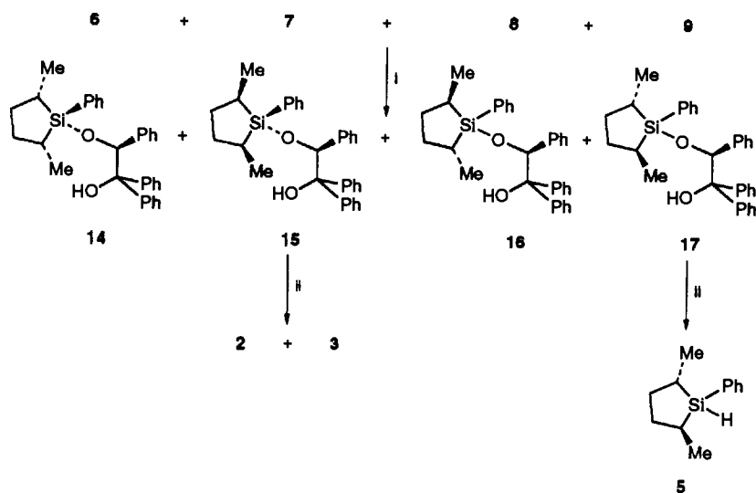
Scheme 2 Reagents and conditions: i, (S)-TPED, imidazole, DMAP in DMF, room temp.; ii, LiAlH 4 in THF, room temp.
