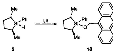
Scheme 3 Reagents and conditions: i, CuCl 2 in MeCN, reflux; ii, 9-anthrylmethanol, imidazole, DMAP in DMF, 40 °C
