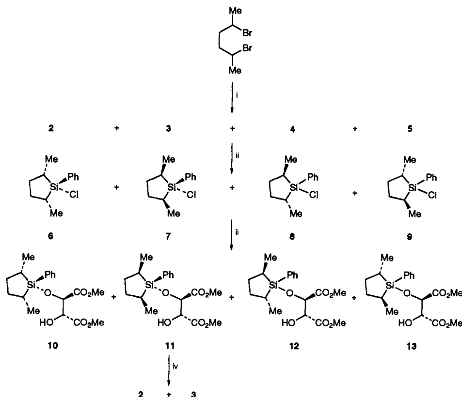
Scheme 1 Reagents and conditions: i, \text{PhSi(H)Cl}_2 , Mg in THF; ii, \text{CuCl}_2 in MeCN, reflux; iii, L-DMT, imidazole in DMF, room temp.; iv, \text{LiAlH}_4 in THF, reflux
