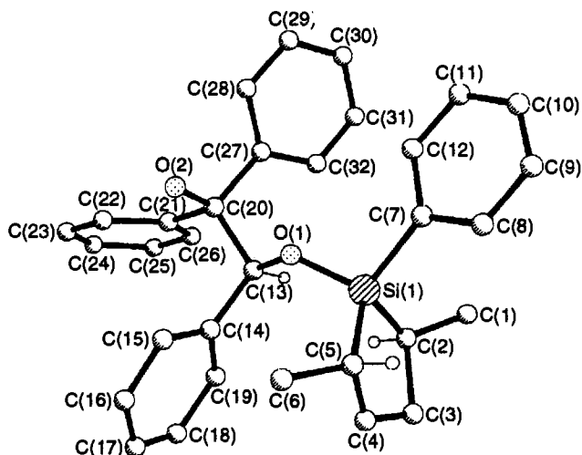
Fig. 2 Molecular structure of the (S,S)-silyl ether 17 derived from (S)-TPED (only selected hydrogen atoms are shown). Selected bond lengths (Å) and bond or torsion angles (°) are as follows: Si(1)–O(1) 1.649(4), Si(1)–C(2) 1.853(9), Si(1)–C(5) 1.884(14), Si(1)–C(7) 1.885(8), Si(1)–O(1)–C(13) 128.5(3), C(2)–Si(1)–C(5) 98.7(5), C(7)–Si(1)–O(1) 105.1(3), C(2)–C(3)–C(4)–C(5) 39.3.
